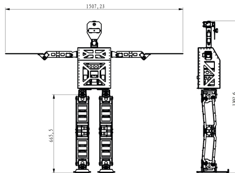
Fig. 2. Robot Dimension
