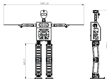
Fig. 2. Robot Dimension
