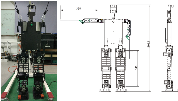
Fig. 1. 1) Strider S1 robots 2) Robot Dimension
