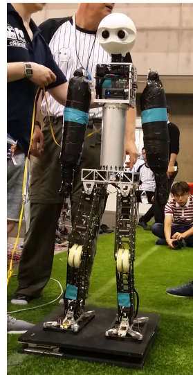
Fig. 3. Copedo robot.
