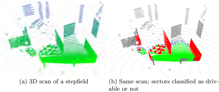
Fig. 8: Example of a 3D scan of the laser range finder.
