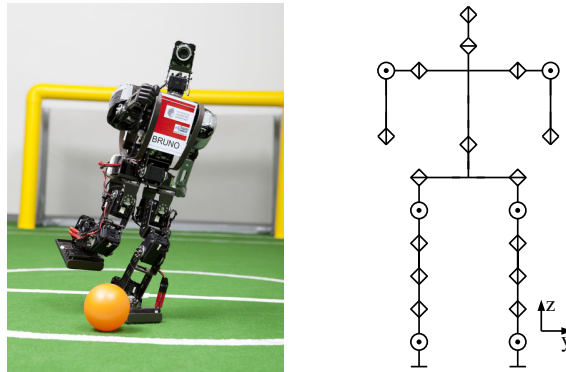
Autonomous humanoid robot Bruno kicking a ball (left, ©K. Binner) and kinematic structure of the robot (right).
