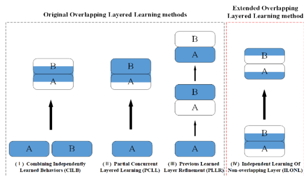
Fig. 2. Independent Learning Of Non-overlapping Layer
